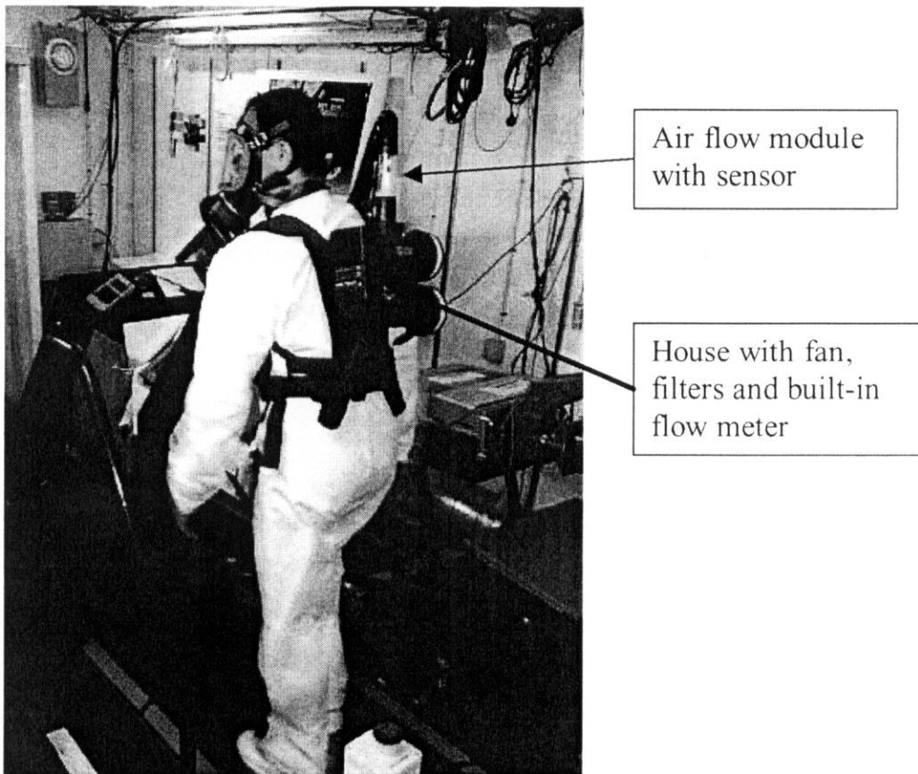
Figure 2. Experimental setup in climatic chamber with treadmill for graded exercise levels. Fan and filter are worn in a separate house on the back. Full face mask is connected to the house via a flexible tube. At the tube end nearest to the house a separate flow meter was mounted.
